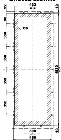
TEMPLATE FOR RECESSED / SEMI-RECESSED AND EXTERNAL MOUNTING
