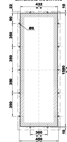
TEMPLATE FOR RECESSED / SEMI-RECESSED AND EXTERNAL MOUNTING
